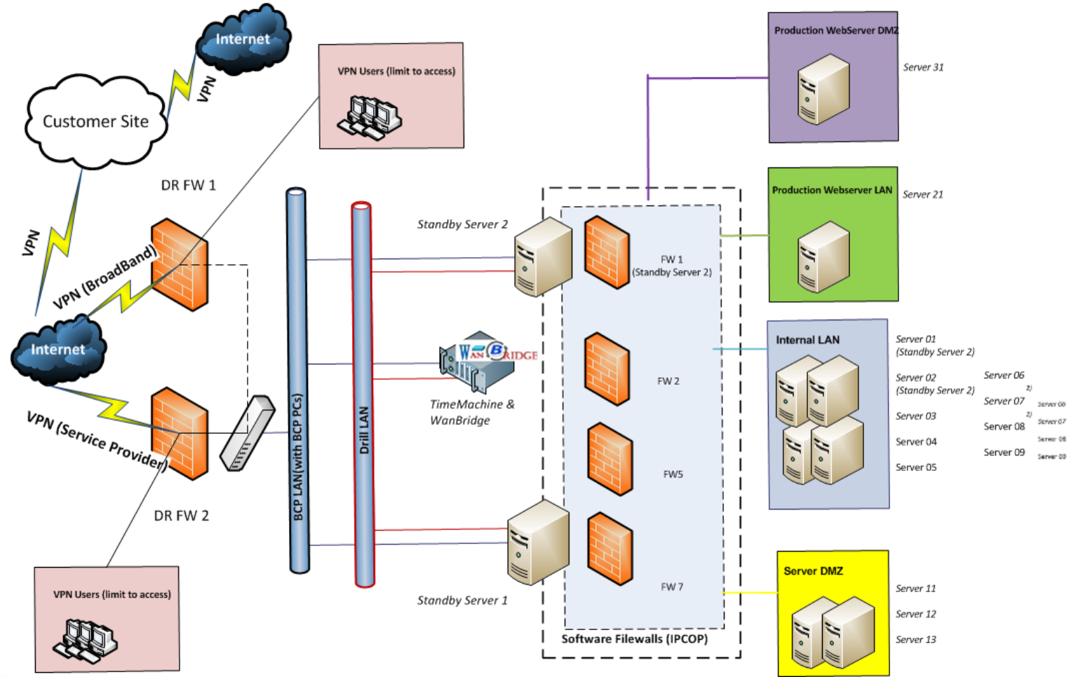
Company A Network Diagram – DR Overview (Final design in DR Site)
